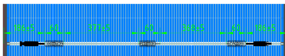
Figure 8. Position of junction box of framed module
