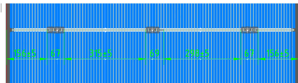
Figure 8. Position of junction box of framed module
