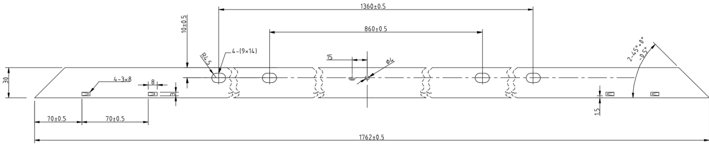
Figure 5. Position of mounting holes of MAGNUS module
