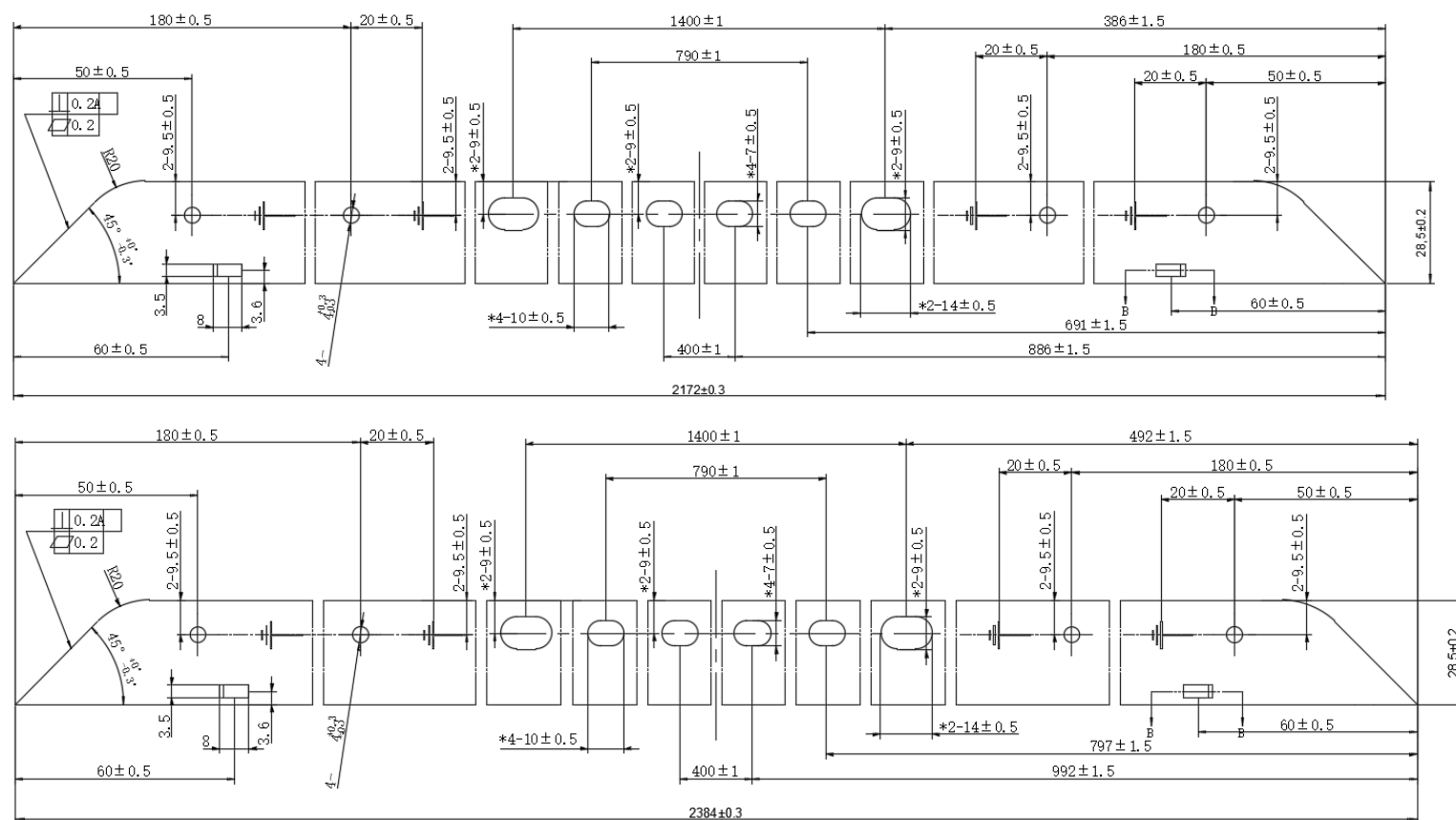
Figure 6. Position of mounting holes of Forza 650 W and 730 W modules
