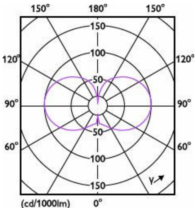
Light Distribution Diagram - CorePro LED HPL/SON M 6Klm 31W 840 E40FR
