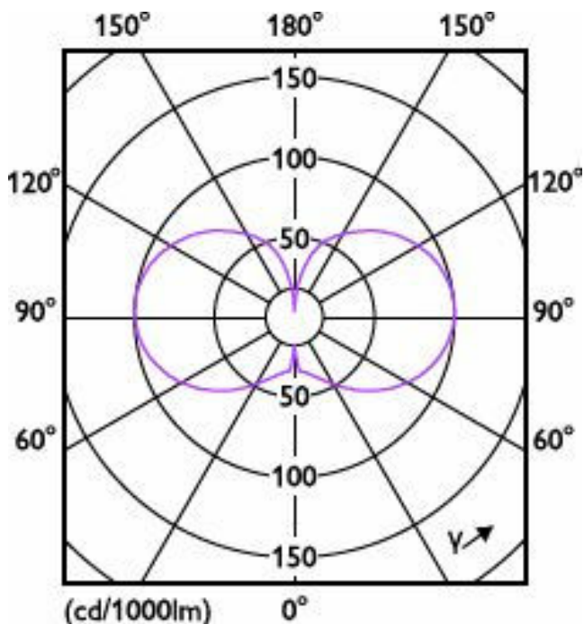
Light Distribution Diagram - CorePro LED HPL/SON M5.5Klm29.5W830E40FR
