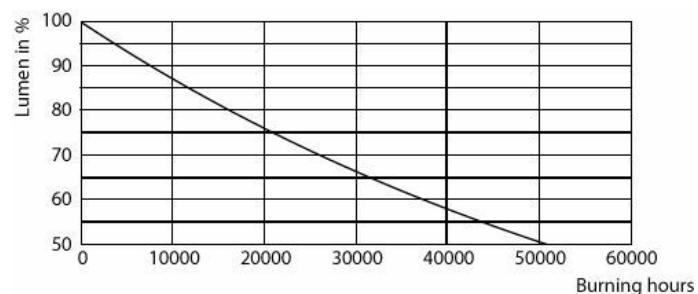
Lumen Maintenance Diagram - CorePro LED HPL/SON M5.5Klm29.5W830E40FR
