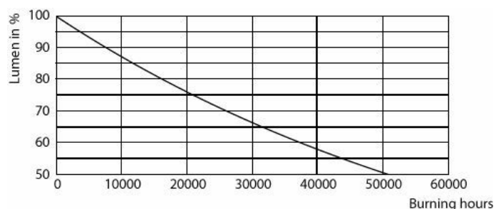
Lumen Maintenance Diagram - CorePro LED HPL/SON M5.3Klm28.5W827E40FR
