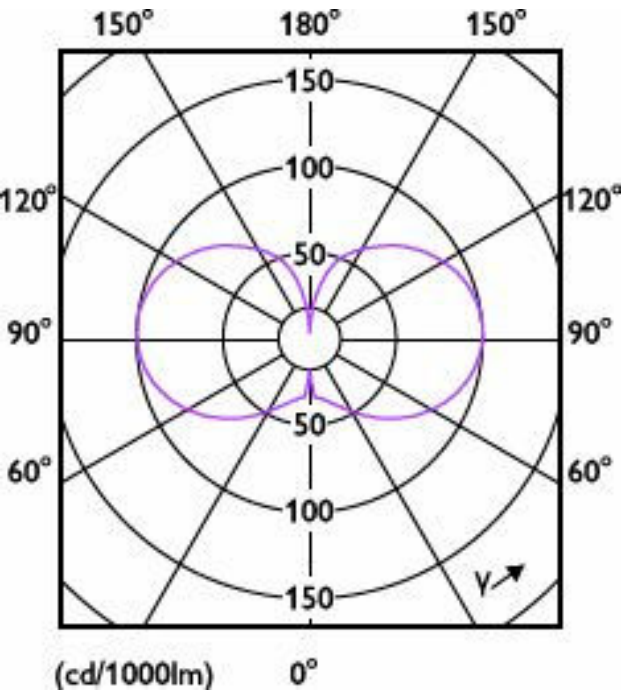
Light Distribution Diagram - CorePro LED HPL/SON M5.3Klm28.5W827E40FR
