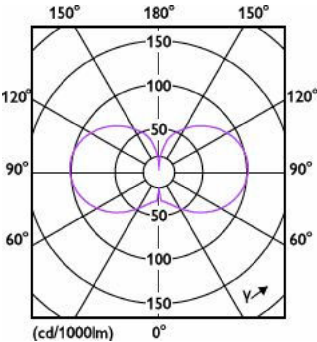
Light Distribution Diagram - CorePro LED HPL/SON M5.5Klm29.5W830E27FR
