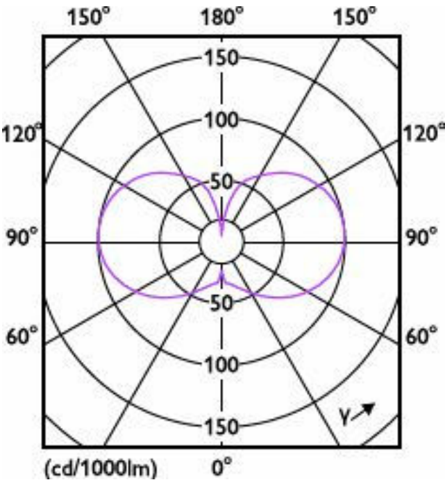
Light Distribution Diagram - CorePro LED HPL/SON M 4Klm 23W 830E27 FR
