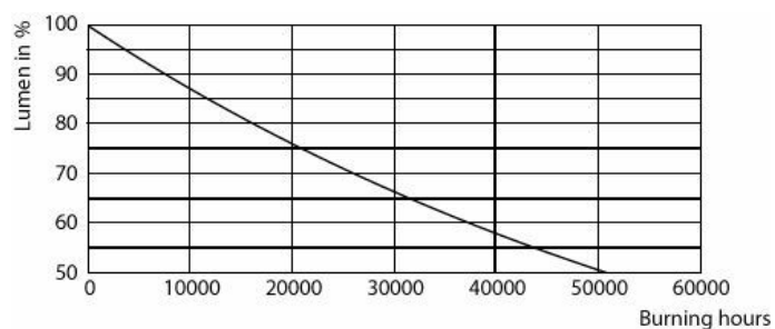
Lumen Maintenance Diagram - CorePro LED HPL/SON M 4Klm 23W 830E27 FR
