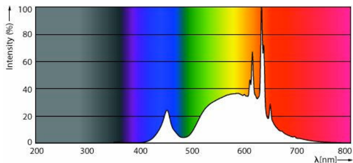
Spectral Power Distribution Colour - CorePro LED HPL/SON M 4Klm 23W 830E27 FR
