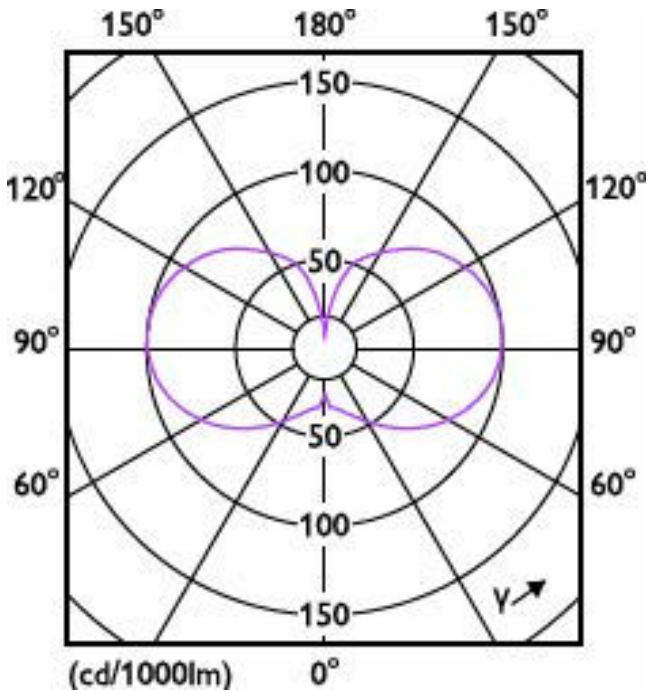
Light Distribution Diagram - CorePro LED HPL/SON M 3.6Klm23W 827E27FR
