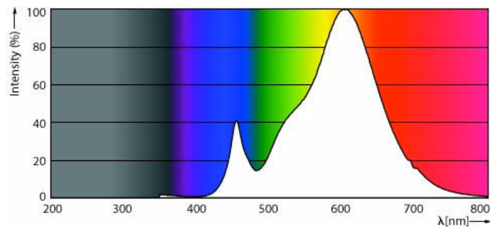
Spectral Power Distribution Colour - CorePro LED HPL/SON M 3.6Klm23W 827E27FR
