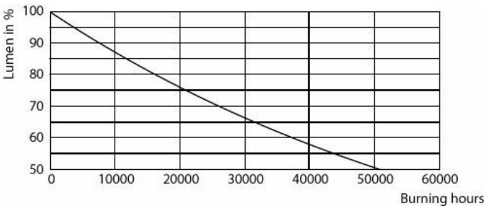
Lumen Maintenance Diagram - CorePro LED HPL/SON M 3.6Klm23W 827E27FR
