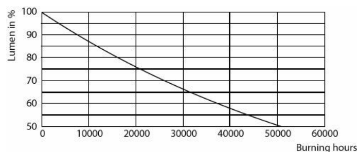
Lumen Maintenance Diagram - CorePro LED HPL/SON M3Klm18.3W840E27FR
