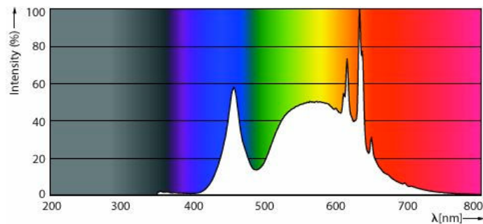
Spectral Power Distribution Colour - CorePro LED HPL/SON M3Klm18.3W840E27FR
