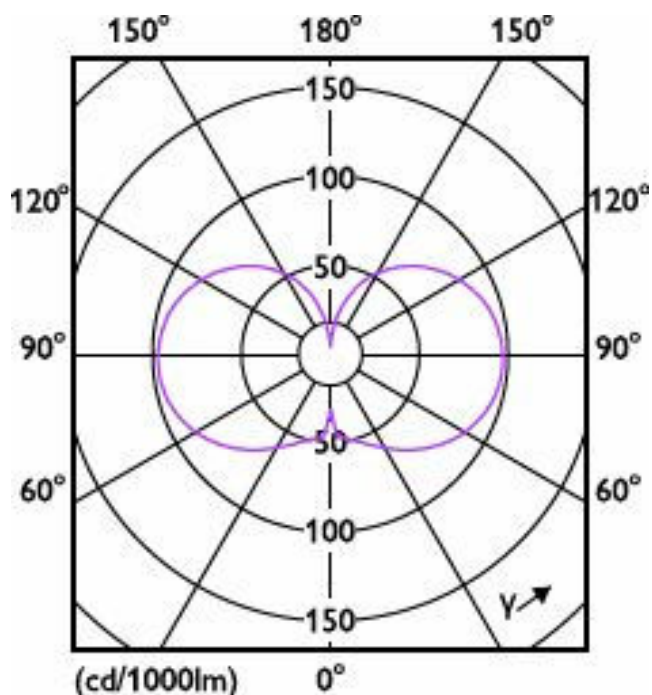
Light Distribution Diagram - CorePro LED HPL/SON M3Klm18.3W840E27FR
