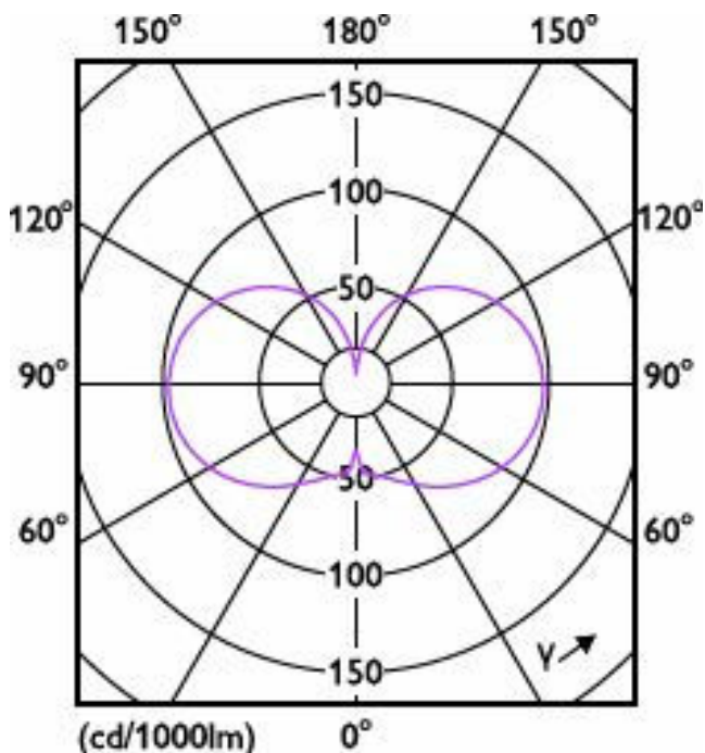
Light Distribution Diagram - CorePro LED HPL/SON M2.6Klm18.3W827E27FR
