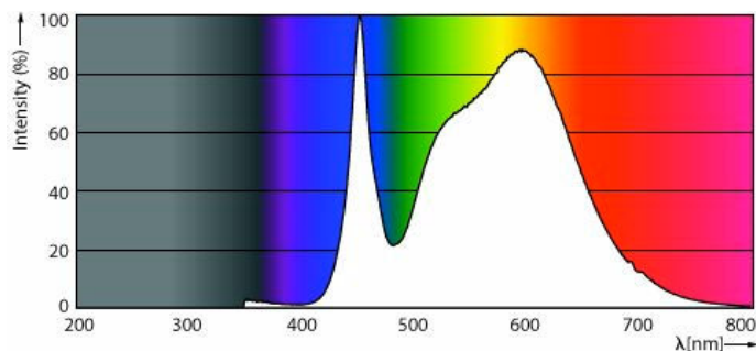
Spectral Power Distribution Colour - CorePro LED HPL/SON M 2Klm13W840E27 FR
