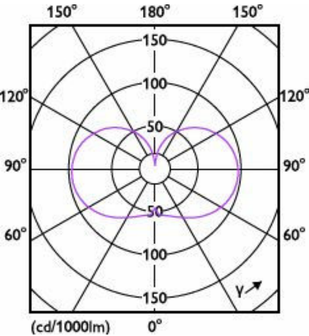
Light Distribution Diagram - CorePro LED HPL/SON M 2Klm13W840E27 FR
