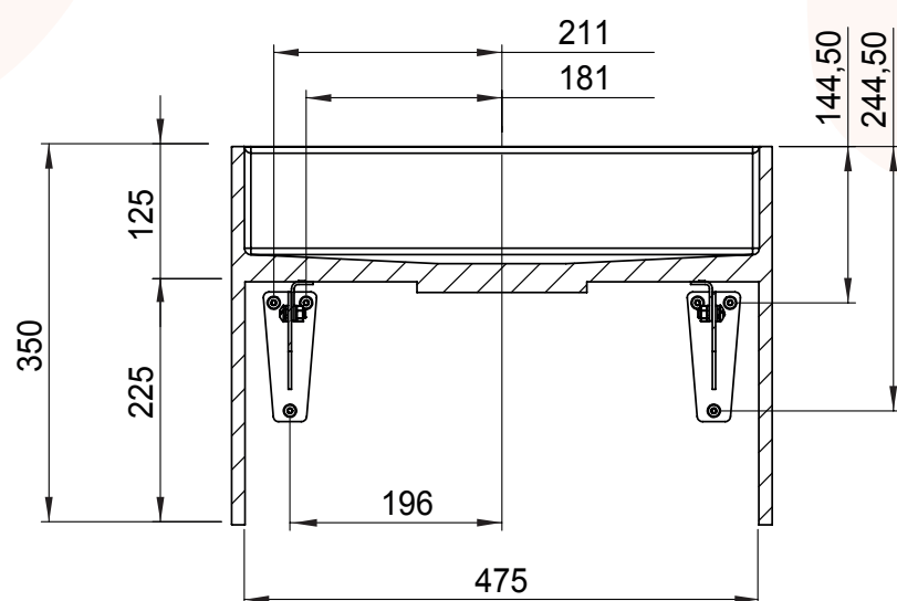
SECTION B-B
