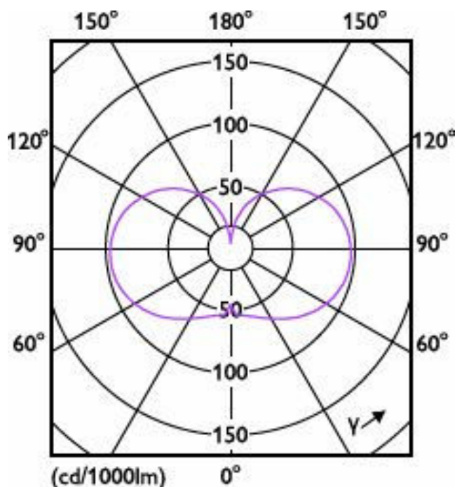
Light Distribution Diagram - CorePro LED HPL/SON M 2Klm13W830E27 FR
