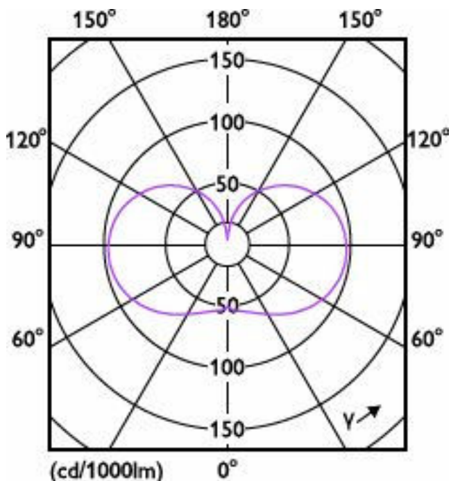
Light Distribution Diagram - CorePro LED HPL/SON M 1.8Klm13W827E27 FR
