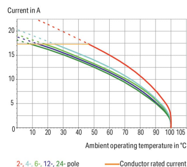
Derating Curve 1-conductor female connector (734-102) with THT male header (734-132) Pin spacing: 3.5 mm / Conductor cross-section: 1.5 mm² "f-st" Based on: EN 60512-5-2 / Reduction factor: 0.8
