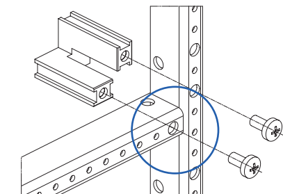
Fig. 5: Support rail connector half (type EPTV05) - for vertical installation
