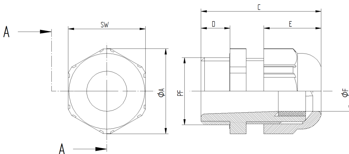
Dimension table:
