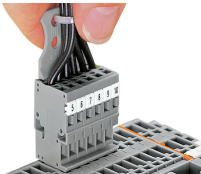
Removing a female plug via conductor bundle provided with strain relief plate.
