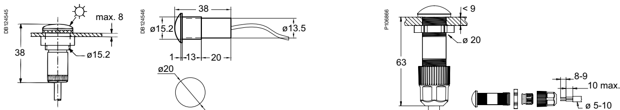
Standard switchboard cell (15281) Fixed externally in vertical position by 2 ø 4 mm screws
