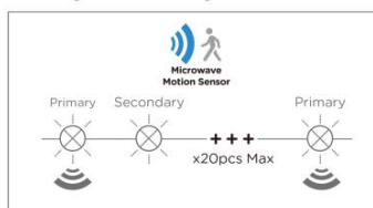
Primary & Secondary connection
