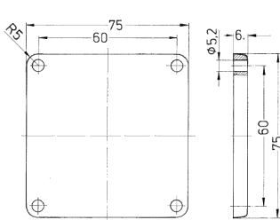
Drawing 1 MB 373 Dim. in mm
