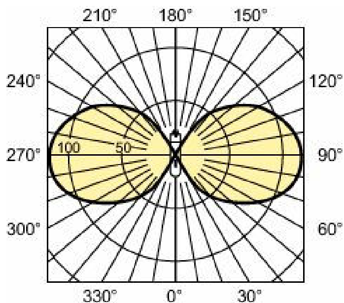
Light Distribution Diagram - MASTER SDW-T 50W/825 PG12-1 1SL/12
