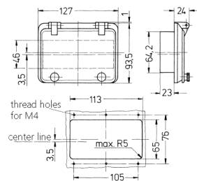
Drawing 6 MB 17 Dim. in mm
