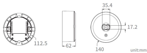
Surface Mount
