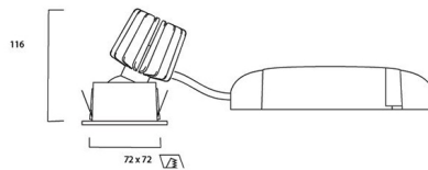
Dimensions (mm)
