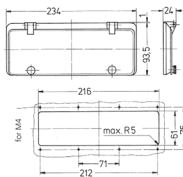
Part no. 40980 / Draw. 6 MB 14 / 12 modules
