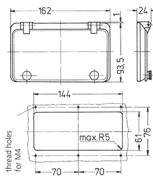
Part no. 40978 / Draw. 6 MB 15 / 8 modules
