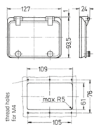
Part no. 40985 / Draw. 6 MB 16 / 6 modules
