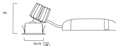
Dimensions (mm)
