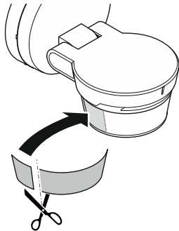
Fig. 24: Glueing the detection range
