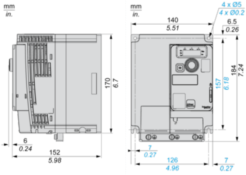
Right View, Front View and Front View with EMC Plate
