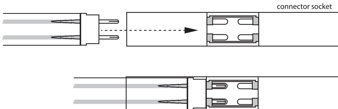
connector socket
