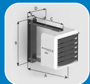
Suspension with U-brackets, art. no. GA8610
