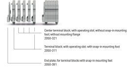
Example of a 5-pole terminal strip, with operating slots, with snap-in mounting foot, cable number = 2
