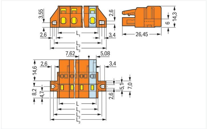
Dimensions in mm L = (\text{pole no.} - 1) \times \text{pin spacing} + 5.08 \text{ mm} L1 = L + 3 \text{ mm} L2 = L + 8.8 \text{ mm} L3 = L + 14.8 \text{ mm} 2- to 3-pole female connectors – one latch only
