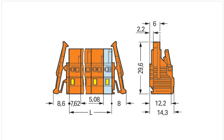
Dimensions in mm L = (pole no. – 1) x pin spacing + 5.08 mm 2- to 3-pole female connectors – one latch only
