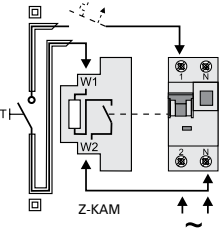
Connection diagram: RCBO-2p, RCBO feed below
