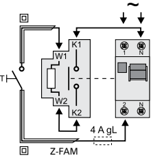
Connection diagram: RCCB-2p, RCCB feed above
