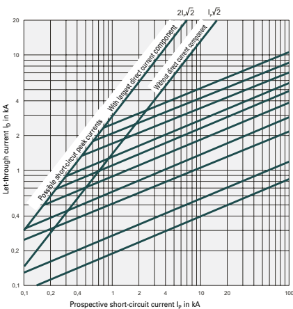
Let-through characteristics of Z-D0-Fuse-Links 2 ... 63A gG(gL)
