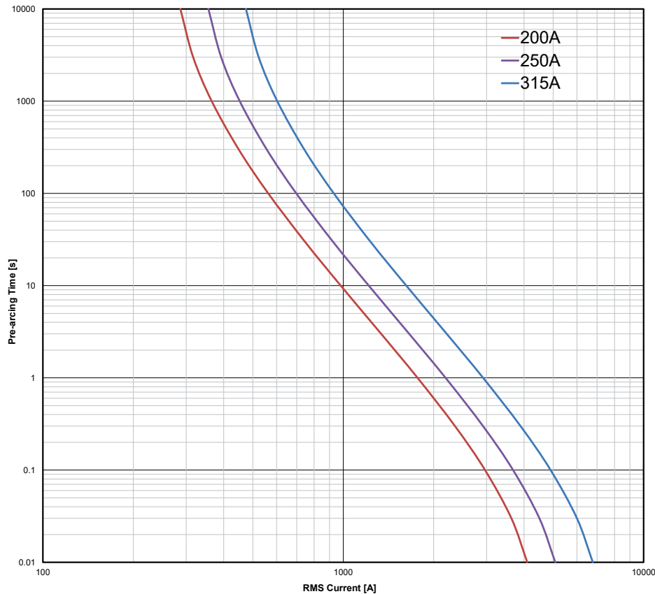
Time-current curve size 3 - 200 A to 315 A
