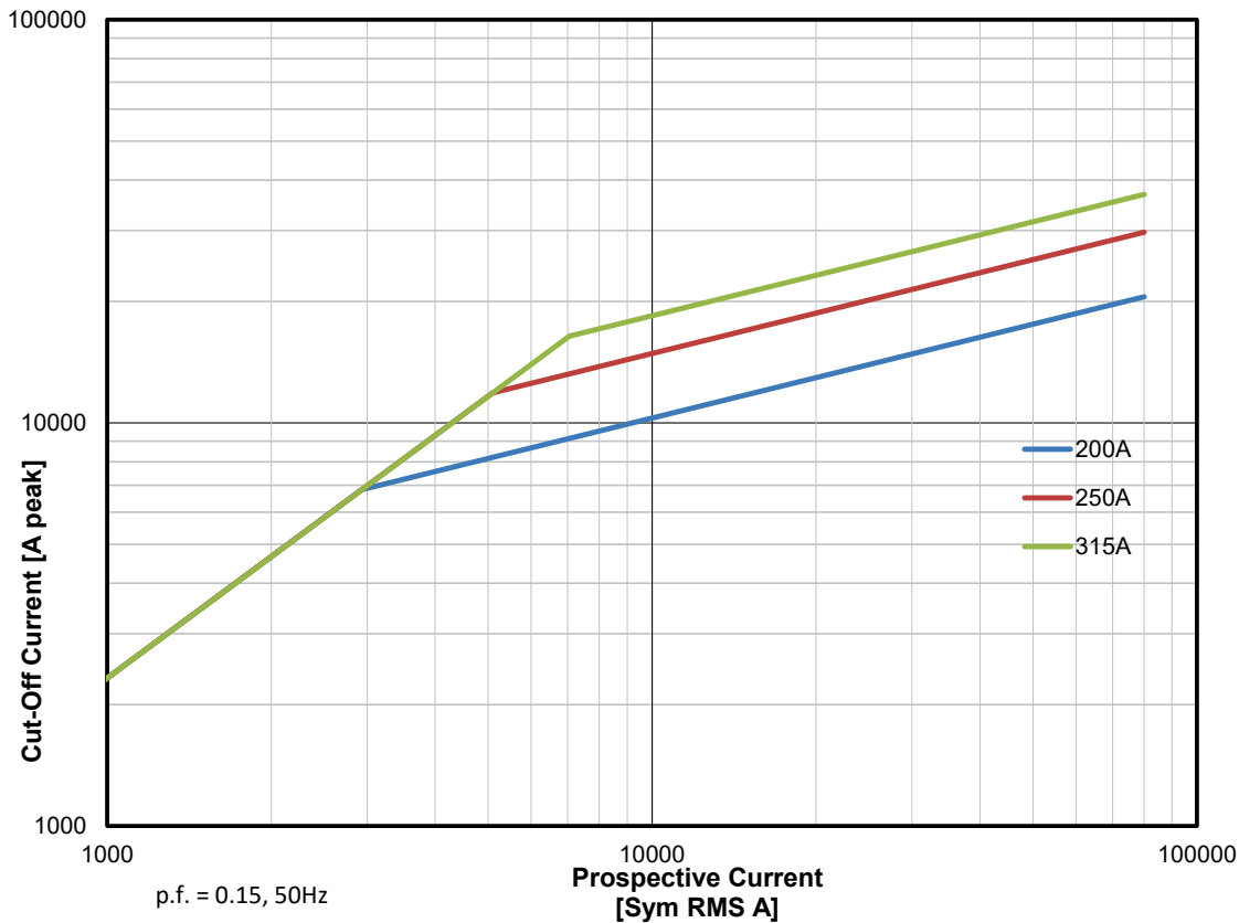
Cut-off curve size 3 - 200 A to 315 A
