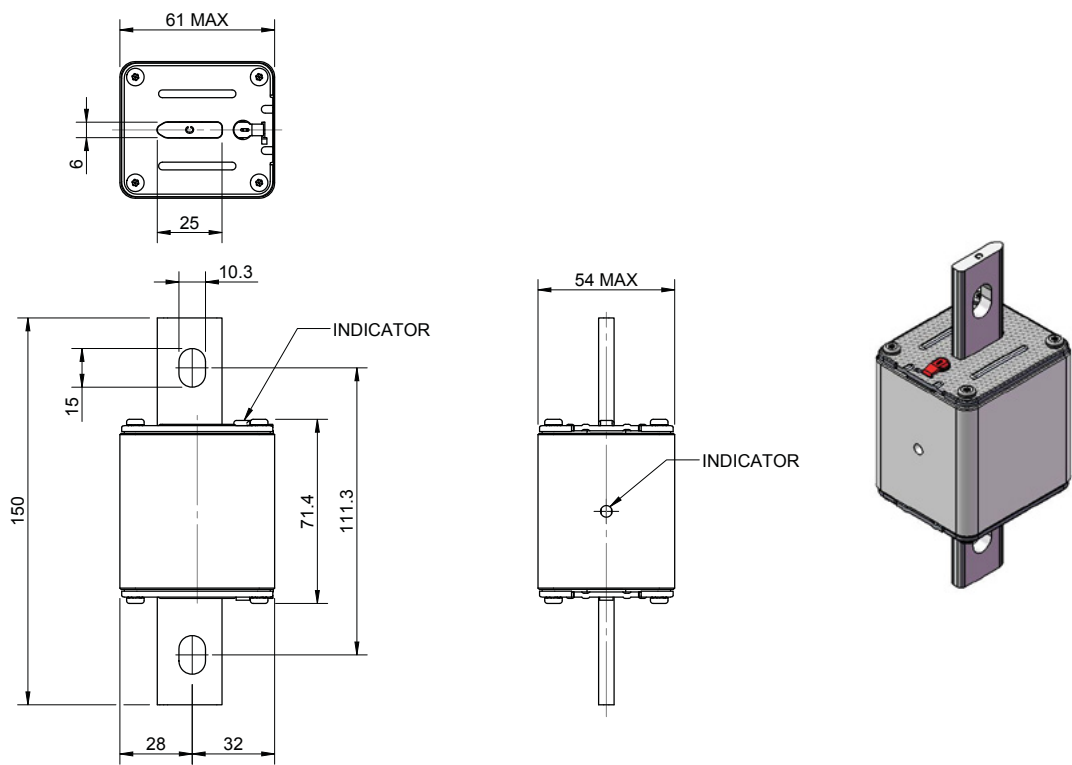
Dimensions (mm) NH2 Blade with bolt holes
