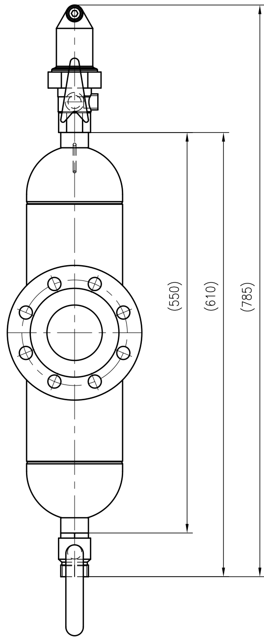
Side view
