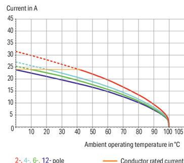
Derating Curve 2-conductor female connector (721-2205/026-000) with THT male header (721-262/001-000) Pin spacing: 7.5 mm / Conductor cross-section: 2.5 mm 2 *f-st* Based on: EN 60512-5-2 / Reduction factor: 0.8
