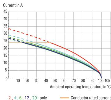
Derating Curve 1-conductor female connector (2721-102/026-000) with THT male header (721-162/001-000) Pin spacing: 5 mm / Conductor cross-section: 2.5 mm² "f-st" Based on: EN 60512-5-2 / Reduction factor: 0.8
