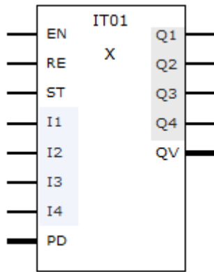
Programme principal
