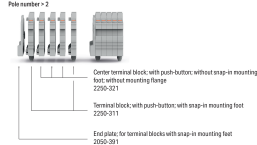
Example of a 5-pole terminal strip; with push-buttons; with snap-in mounting feet File number: 2
