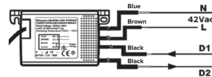
Fig. 3: Connection diagram
