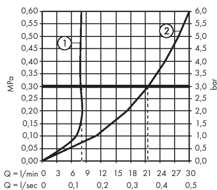
AXOR One 48440XXX
