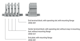
Example of a 4-pole terminal strip; with operating slot; with mounting flange
