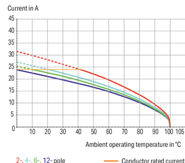
Derating Curve 2-conductor female connector (721-2209/026-000) with THT male header (721-262/001-000) Pin spacing: 7.5 mm / Conductor cross-section: 2.5 mm² *f-st* Based on: EN 60512-5-2 / Reduction factor: 0.8
