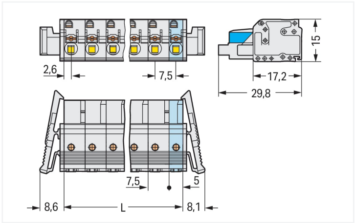
Dimensions in mm L = (pole no. – 1) x pin spacing + 5 mm 2-pole female connectors – one latch only
