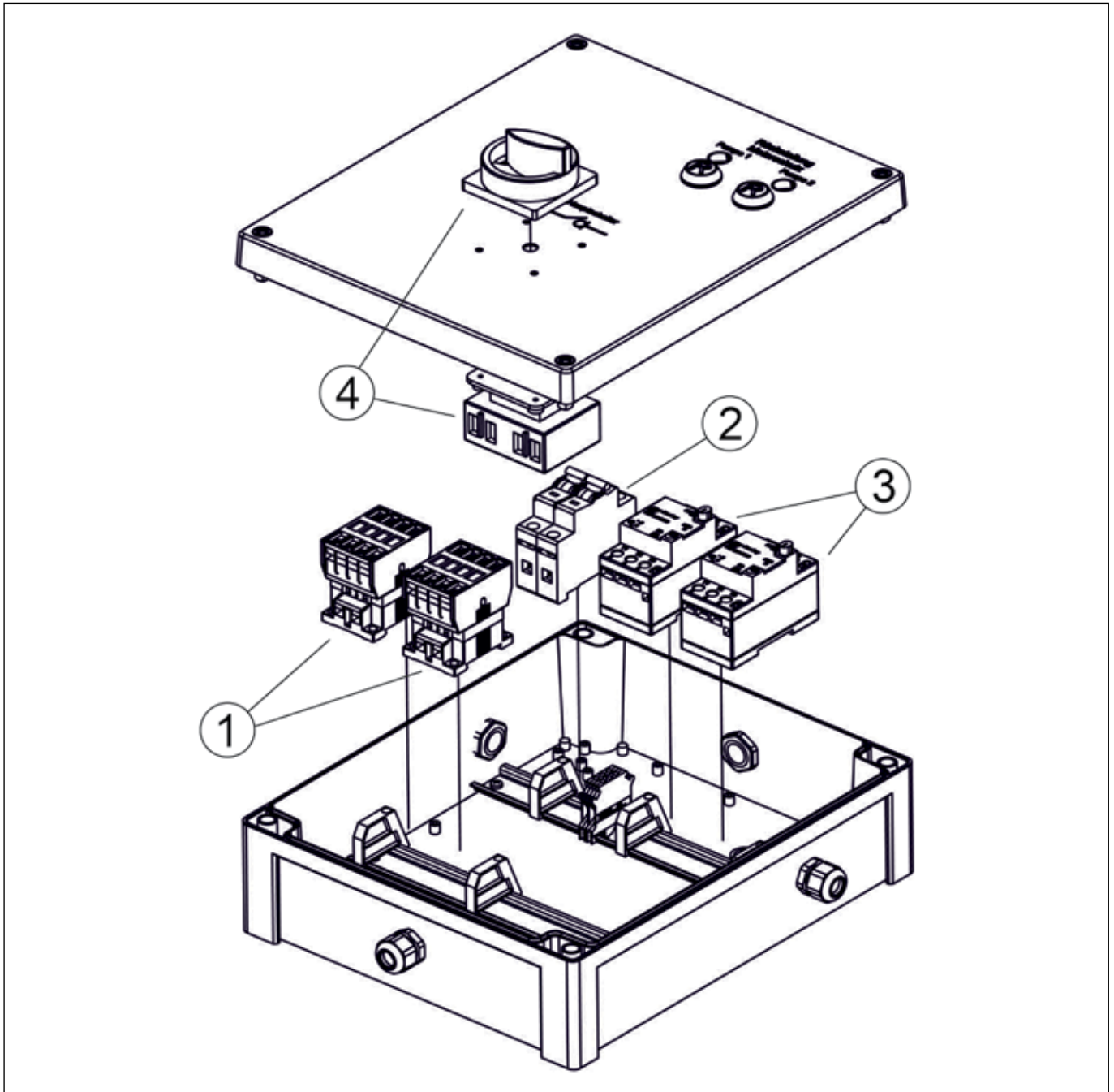
Figure 25: Power section
