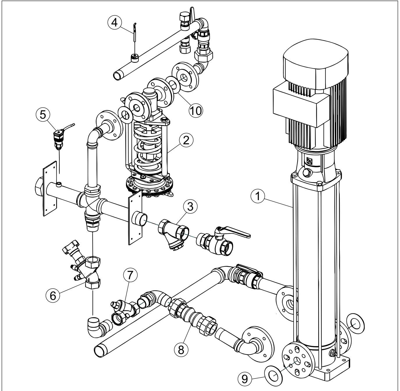
Figure 20: Spare parts for piping
