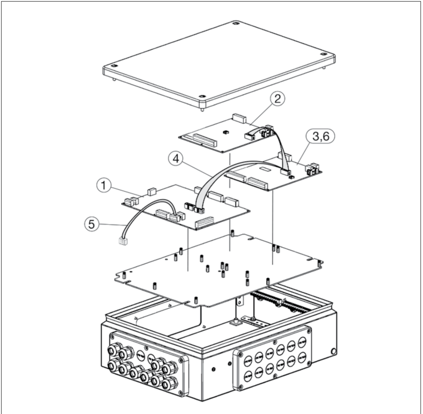
Figure 22: Spare parts switch cabinet
