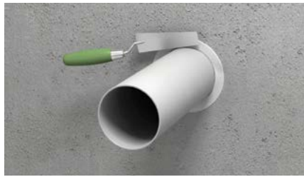
2. Close the gap with loose mineral wool and seal it with a gap filler like Walraven Pacifyre® A acrylic sealant, Pacifyre® H hybrid sealant or Walraven Pacifyre® FPM fire protection mortar (fill depth = 10 mm).
