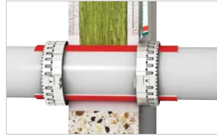
■ Built-in situation flexible walls \geq 100 mm
