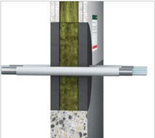
■ Wall penetrations with composite plastic pipes including aluminium up to Ø 32 mm EI 120 U/C.
