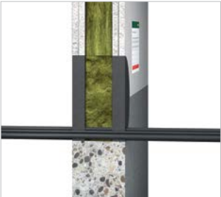
■ Wall penetrations with sheathed cables up to 21 mm or cable bundles up to 50 mm EI 120.
