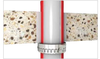
■ Built-in situation ceilings \geq 150 mm
