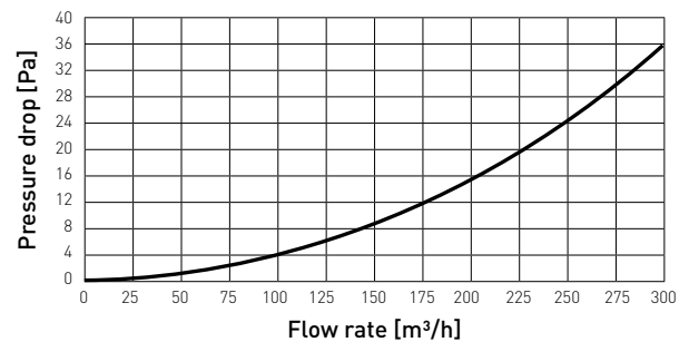
Specifications for supply and extraction
