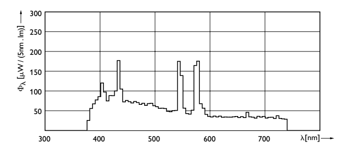
XDPB_XDMSR_575W_SA2-DE-Spectral power distribution B/W
