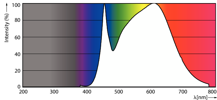
Spectral Power Distribution Colour - MAS LED ExpertColor 7.5-43W MR16 940 24D
